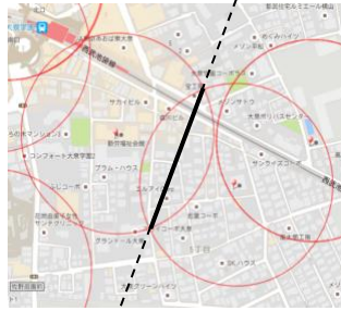
Figure 3. Circular model of the area covered by AEDs
