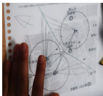
Figure 9. Student’s worksheet: diagram of AEDs
