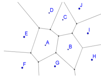
Figure 4. The Voronoi diagram of AEDs
