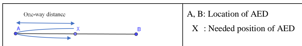
Figure 12. Diagram to consider the installation interval of AED
